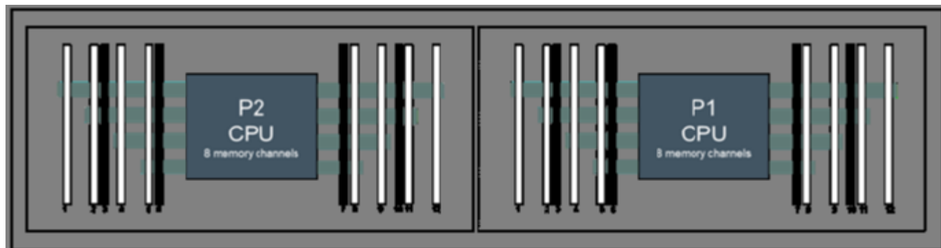
Front of Server HPE ProLiant DL380a Gen11
