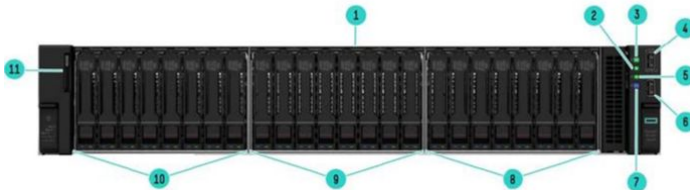
Front View - 24 SFF chassis shown
